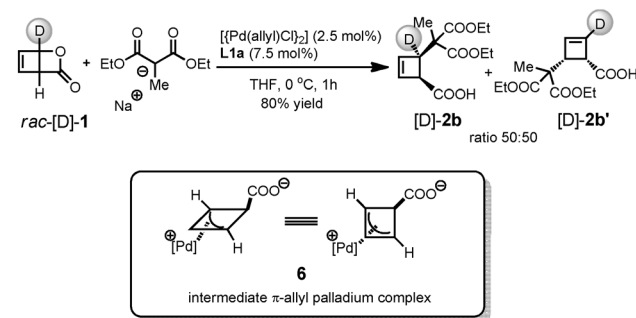
Scheme 7. cis -Selective deuterium labeling experiment employing substrate [D]-1. The yield was determined by NMR spectroscopy (internal standard). See Supporting Information.
