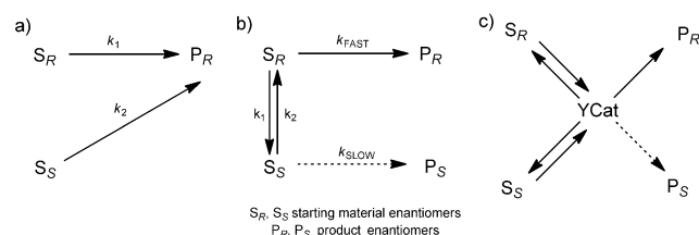
Scheme 1. Strategies for deracemization of a racemate. a) Enantioconvergent process. b) Dynamic kinetic resolution (DKR). c) Dynamic kinetic asymmetric transformation (DYKAT). Dashed arrows represent steps with low rate constant.
