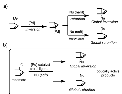
Scheme 2. a) Conventional mechanism and stereochemical outcome of the palladium-catalyzed allylic alkylation (Tsuji–Trost reaction). b) Diastereodivergent deracemization through palladium-catalyzed asymmetric allylic alkylation.
