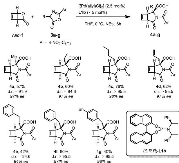
Scheme 5. Scope of azlactone nucleophiles in the cis -selective diastereodivergent deracemization. Yields refer to analytically pure, isolated compounds. The d.r. values were determined by NMR analysis of the crude mixture, and refer to the additional stereocenter.
