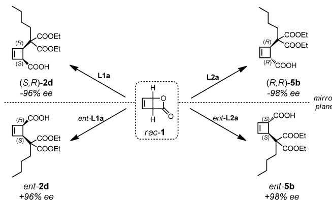
Scheme 9. Preparation of four different products starting from racemic lactone 1 through diastereodivergent deracemization. See the Supporting Information.
