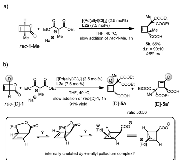
Scheme 8. a) Preparation of a cyclobutyl quaternary center through trans -selective diastereodivergent deracemization. b) trans -selective deuterium labeling experiment employing substrate [D]- 1 . The yield was determined by NMR spectroscopy (internal standard).
