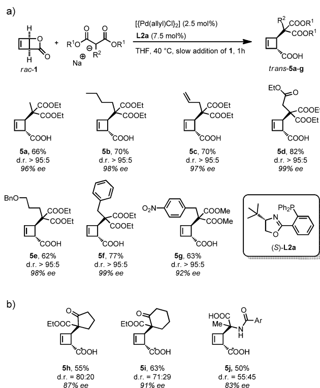
Scheme 6. a) Scope of malonate nucleophiles in the trans -selective diastereodivergent deracemization. The ee values were measured on the corresponding benzamides. The d.r. values were determined by NMR analysis of the crude mixture. b) Scope of additional nucleophiles for the trans -selective process. Yields refer to analytically pure, isolated compounds. The yield of 5j was determined by NMR spectroscopy (internal standard). For 5 and 5i the ee values were determined for the corresponding benzamides, and for 5j on the dimethylester; these values refer to the major diastereoisomer. The d.r. values were determined by NMR analysis of the crude mixture. For 5h , 5i , and 5j , exclusively trans -disubstituted cyclobutenes were obtained, the d.r. values refer to the center marked with *. See Supporting Information.
