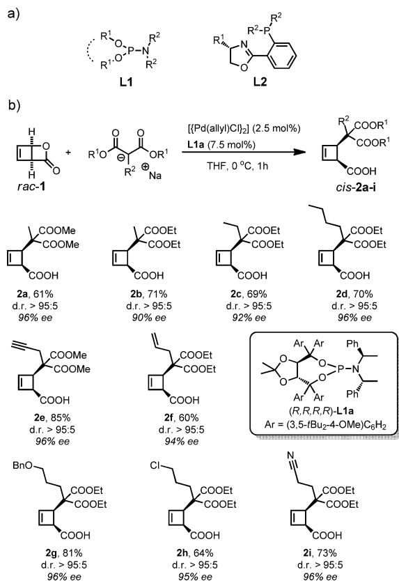
Scheme 4. a) Best-performing chiral ligands for the diastereodivergent deracemization process. b) Scope of malonate nucleophiles in the cis -selective diastereodivergent deracemization. Yields refer to analytically pure, isolated compounds; for compounds 2d , 2e , 2f , 2h the yields were determined by NMR spectroscopy (internal standard). The d.r. values were determined by NMR analysis of the crude mixture. The ee values were determined for the corresponding benzamides (see Supporting Information). For compounds 2c and 2g the reactions were performed using 5 mol% of [\text{Pd}(\text{allyl})\text{Cl}]_2 and 15 mol% L1a .
