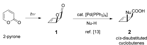
Scheme 3. Palladium-catalyzed diastereoselective synthesis of cyclobutenes.
